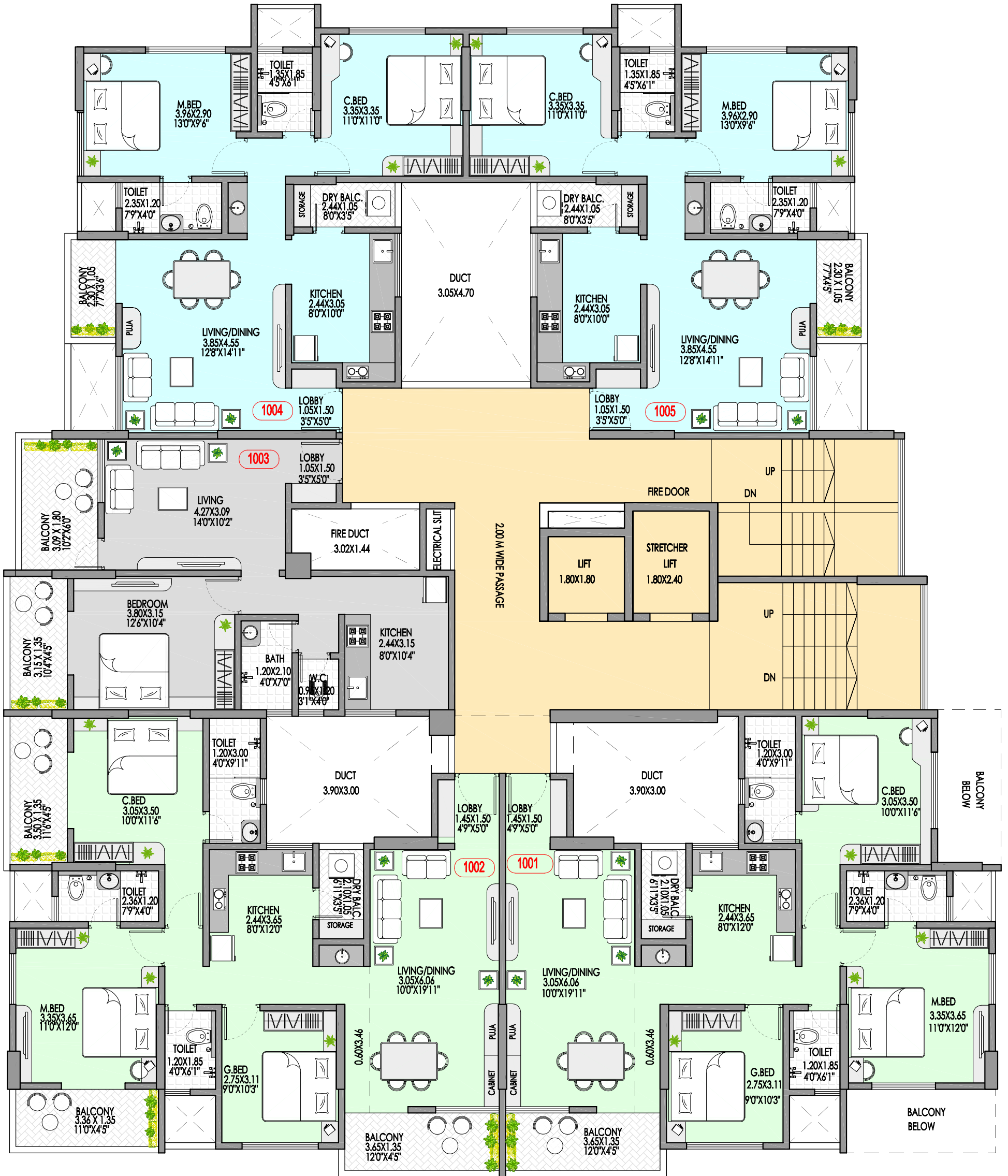
--- 15M WIDE ROAD --- TENTH FLOOR PLAN
