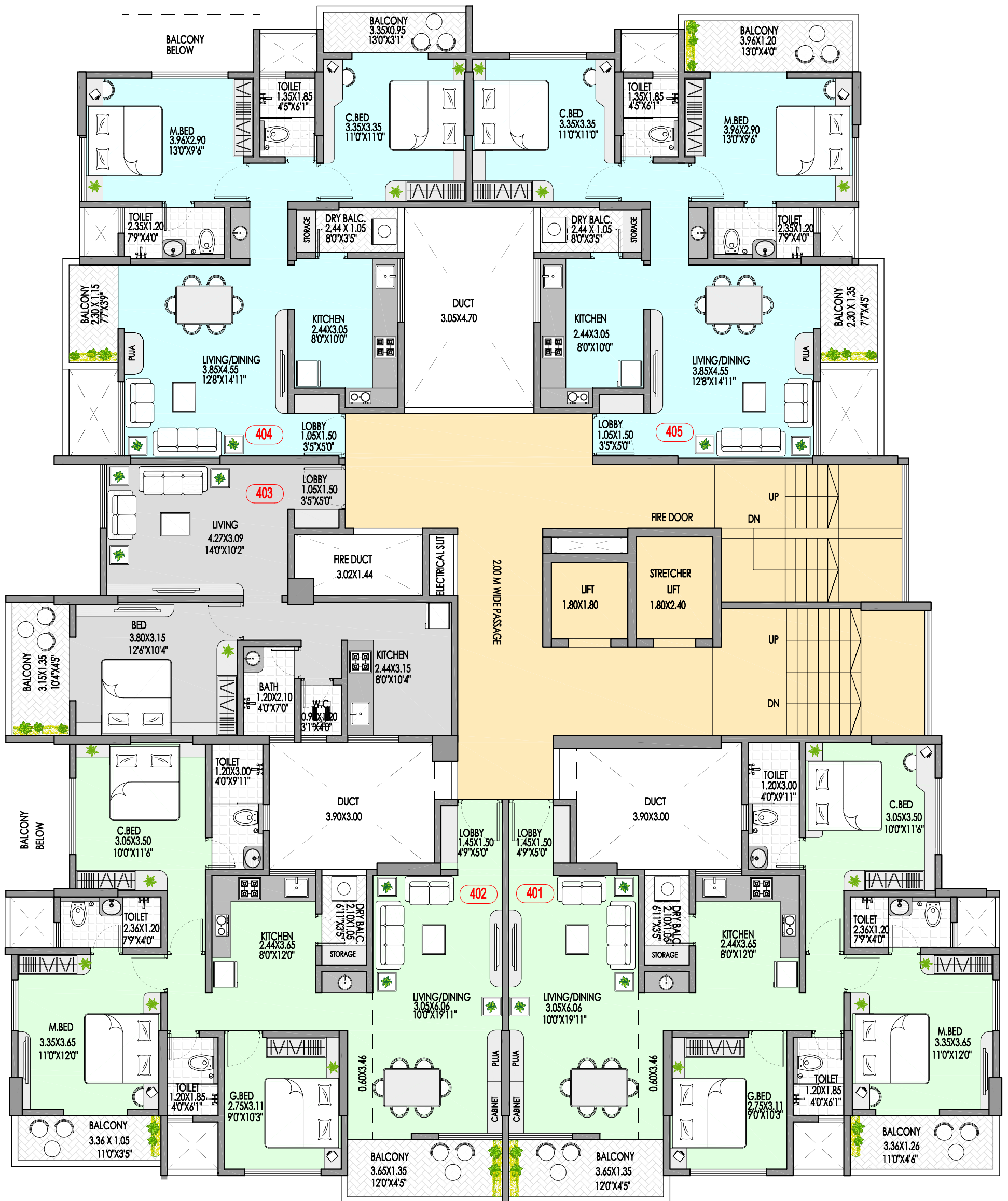
--- 15M WIDE ROAD --- FOURTH FLOOR PLAN
